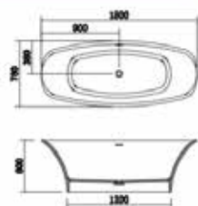
BT6076A SIZE: 1800x760x600mm BT6076B SIZE: 1757x760x600mm
