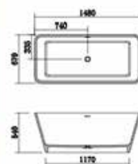
BT6052A SIZE:1480x670x540mm SIZE:1630x710x590mm
