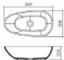
BAI 147 SIZE 560x300x150mm
