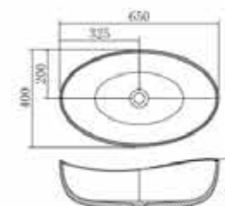
BA1214 SIZE: 650x400x200mm
