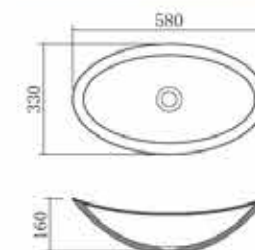
BA1225 SIZE: 580x330x160mm
