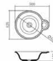
BA1211 SIZE: 500x420x140mm
