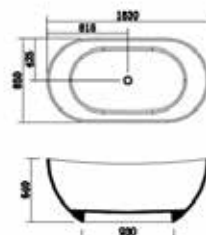
BT6074 SIZE: 1630x850x640mm SIZE: 1800x850x640mm
