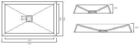
CONCRETE BASIN
