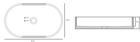
CONCRETE BASIN
