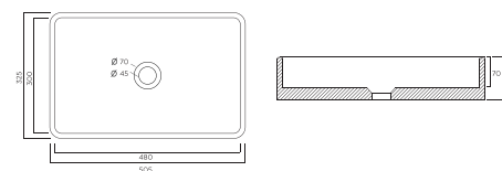
CONCRETE BASIN
